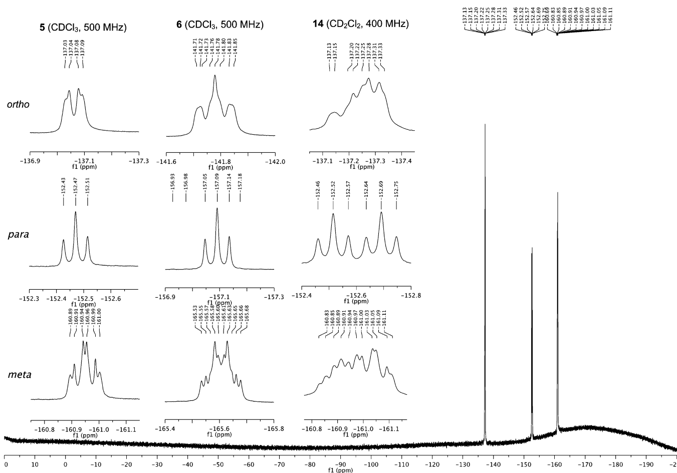
Figure 1. ^{19}\text{F} NMR spectrum of 14 (large spectrum), exhibiting typical chemical shifts for perfluorophenyl groups. Insets show ortho , para , and meta fluorine peaks for compounds 5, 6, and 14.
