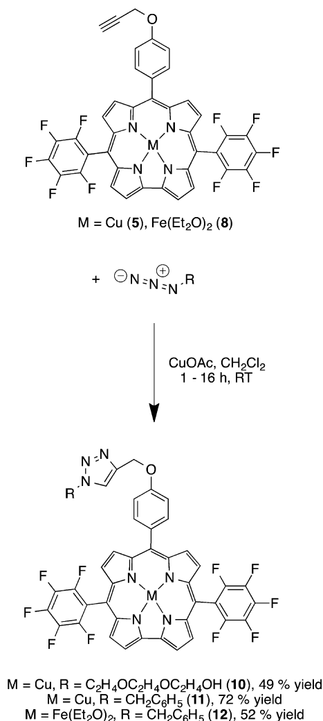
Scheme 2. Test Reactions to Confirm Reactivity of Propargyl-Functionalized Corroles 5 and 8 toward the “Click” Reaction with Small Substrates
